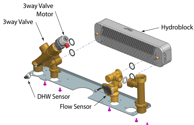
Fig. 2: Hydroblock
