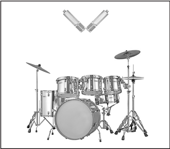
In this diagram, two WA-47jr’s are used in a coincident pair, also known as XY configuration, to record stereo drum overheads.
